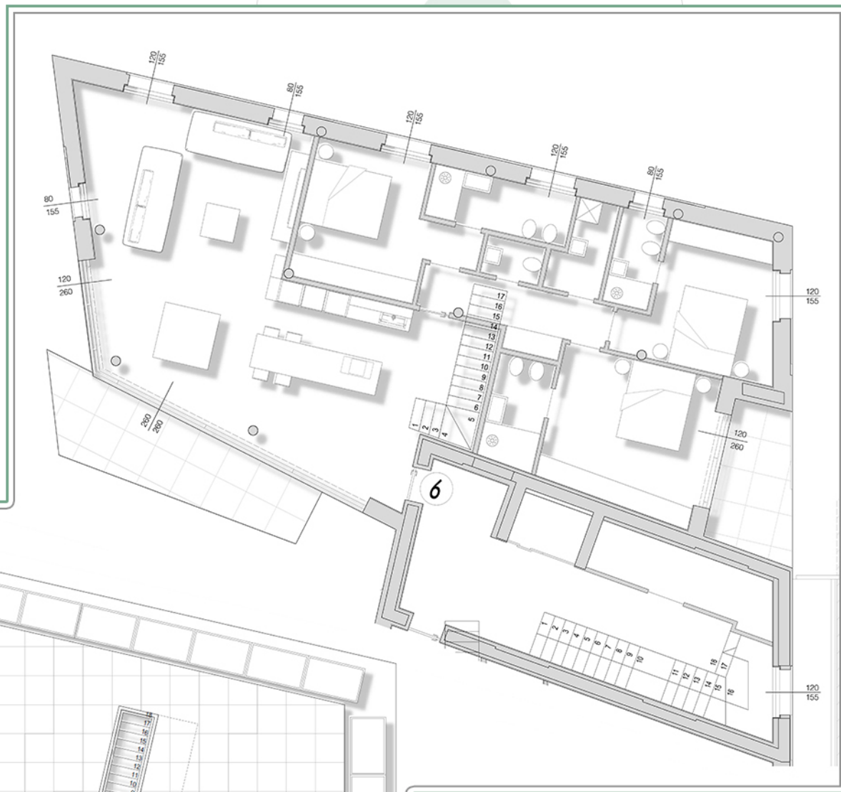
UNIT 6 SECOND FLOOR – + AND TERRACE
